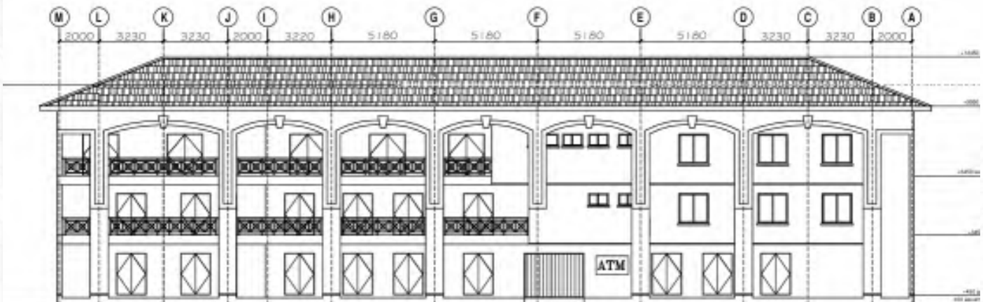
SIDE ELEVATION
